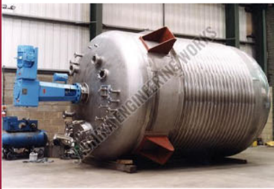
Limpet Coil Reactor
